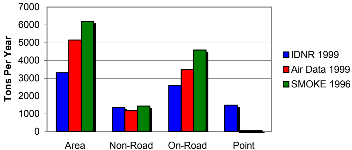
Figure 3: VOC inventory comparison
