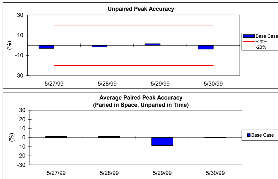
Statistical results using doubled IC/BC concentrations. Metrics are calculated using the methods described in Figure 6.
