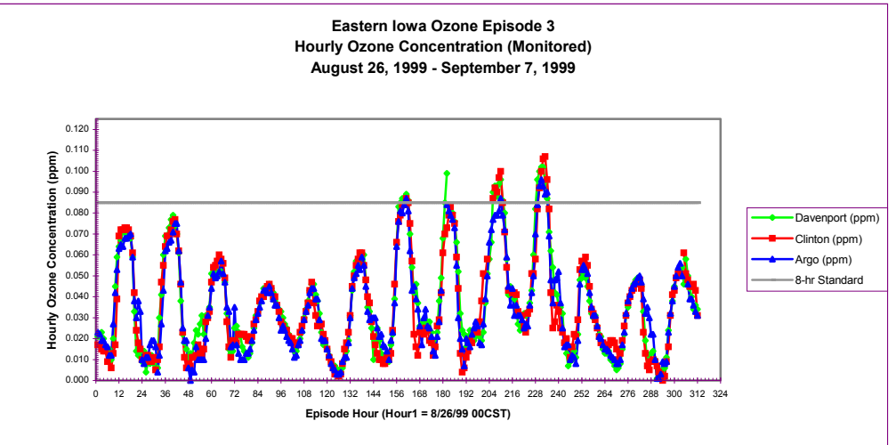
Figure 1. Observed ozone concentrations recorded near the Quad Cities Area. Data used in determining modeling episodes.
