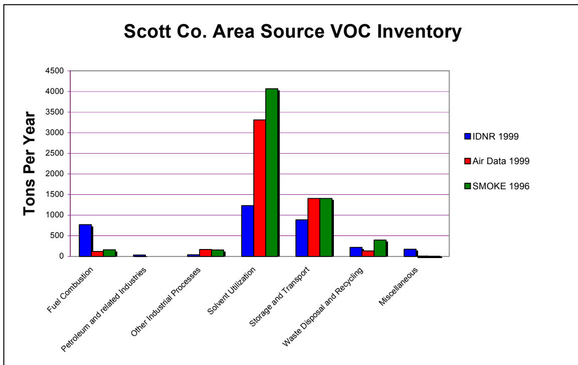
Figure 4: Comparison of VOC sources
